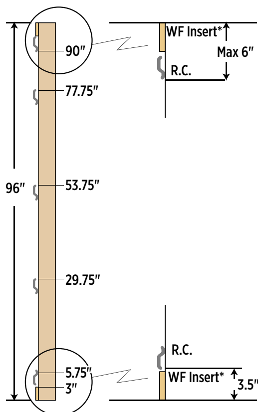
RESILIENT CHANNEL SPACING
